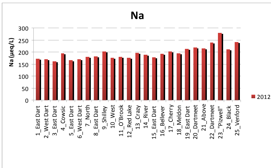
Figure 3. Sodium concentrations for water samples collected in April 2012 from Dartmoor streams
