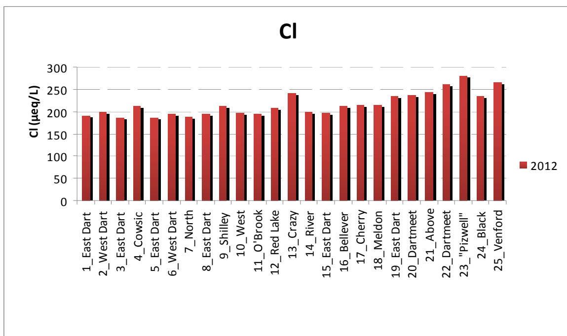
Figure 8. Chloride concentrations for water samples collected in April 2012 from Dartmoor streams
